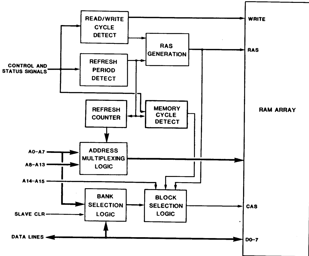
FIGURE 1.1. 2066 BLOCK DIAGRAM
