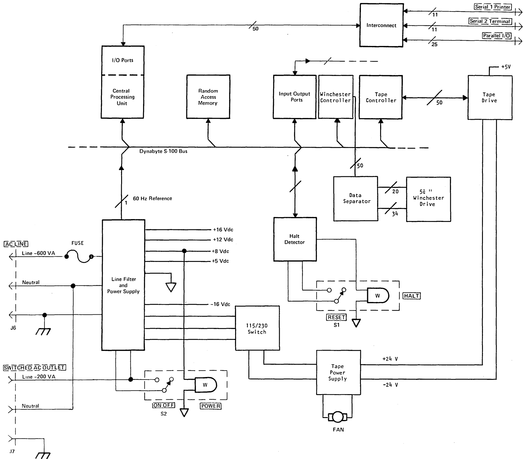
Figure 3.1 5710 Computer Functional Block Diagram
